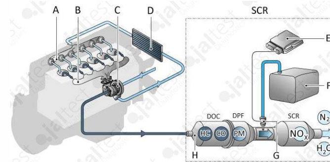
DPF regeneration
