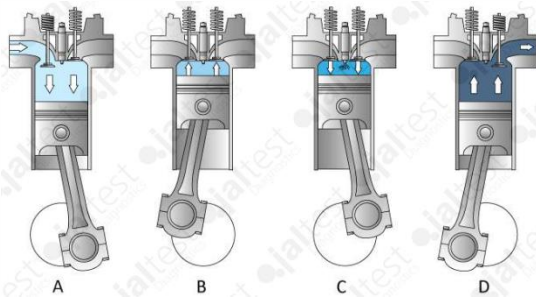
Compression test
